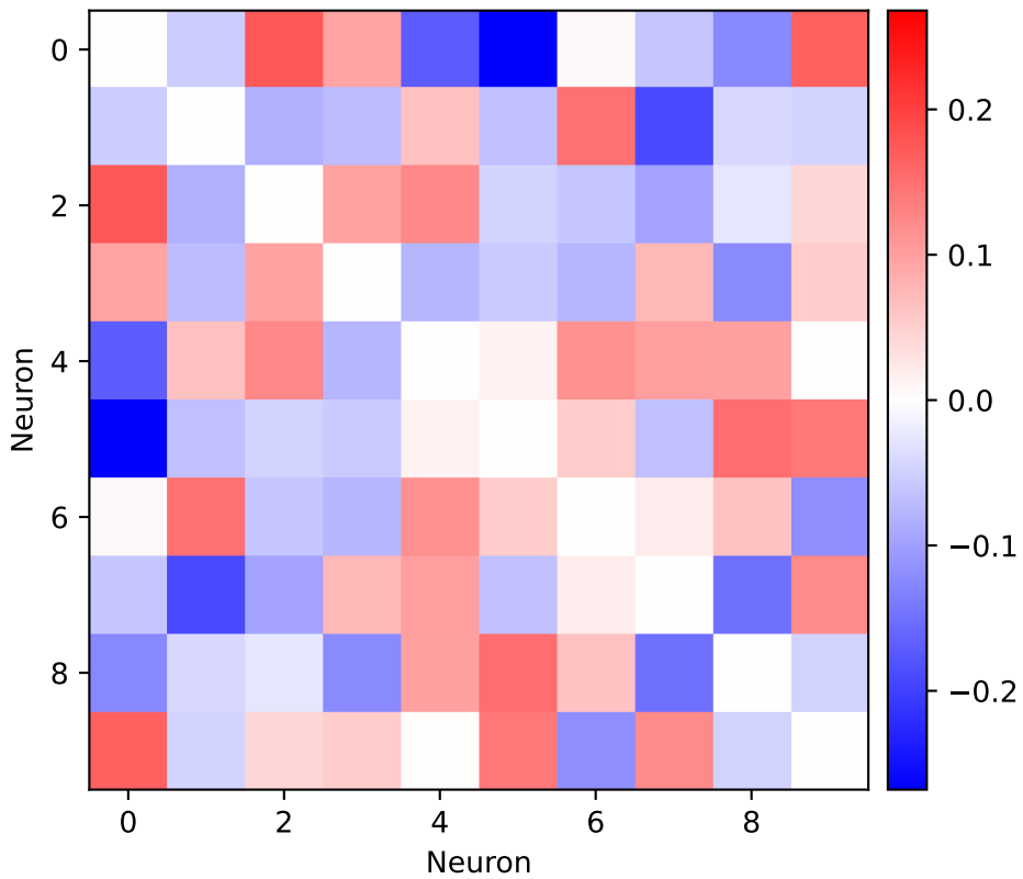
Correlation coefficient matrix
