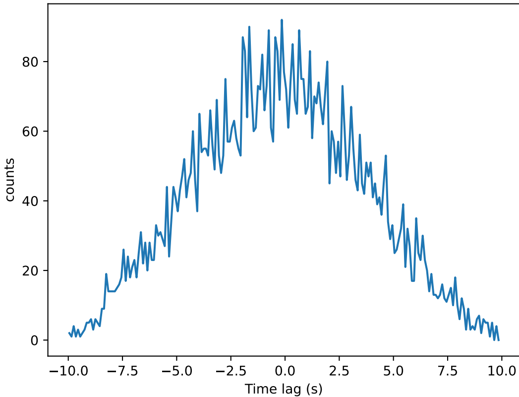
Cross-correlation histogram
